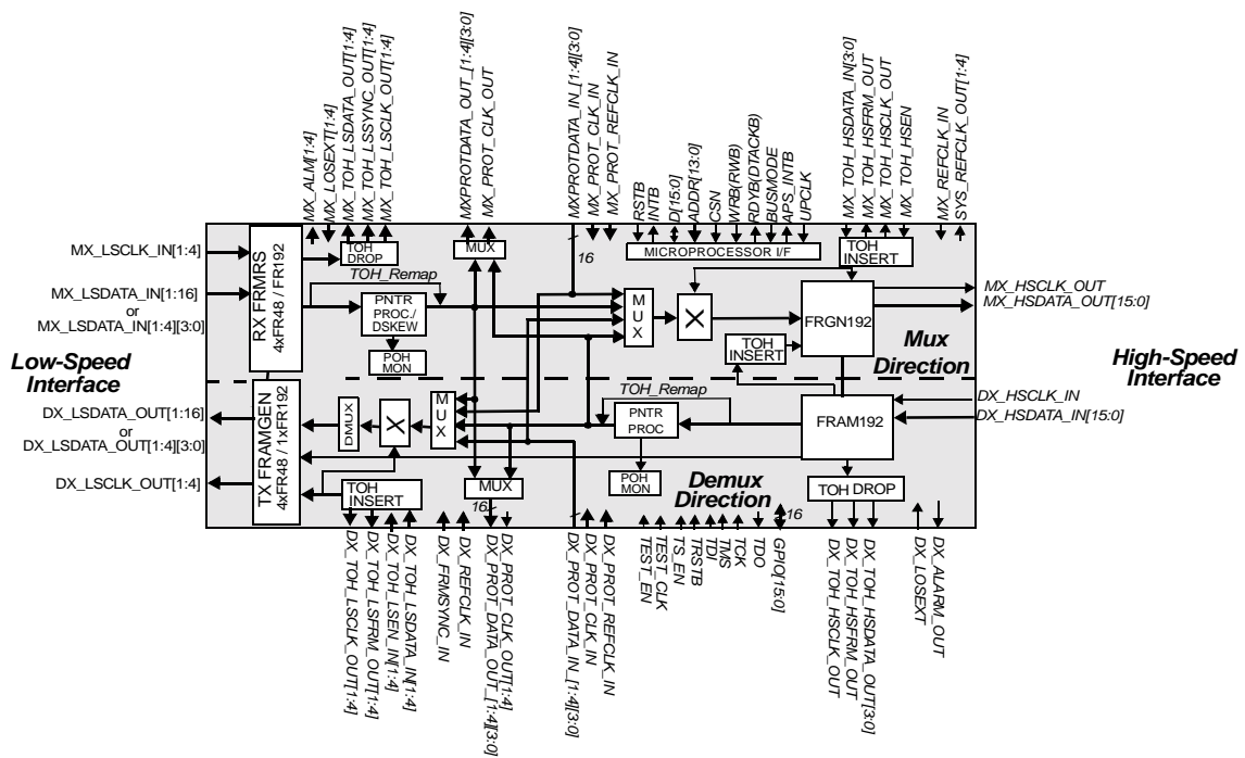
Figure 1: Block Diagram
